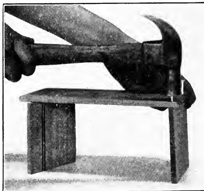
Fig. 288—Nailing End
